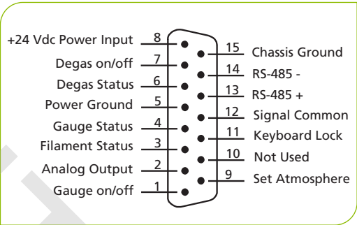
User Interface Connector 15-pin subminiature-D male
