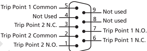
Trip Points Connector 9-pin subminiature-D male
