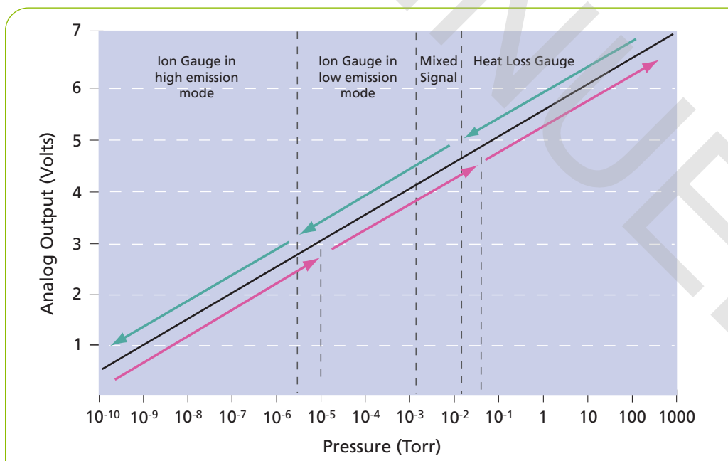
Autoranging switch points and analog output
