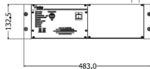
FRONT VIEW ON RVC/DSU/SUBRACK
