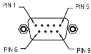
9-pin Type "D" Male Connector
