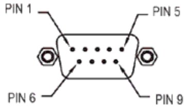
9-pin Type "D" Male Connector
