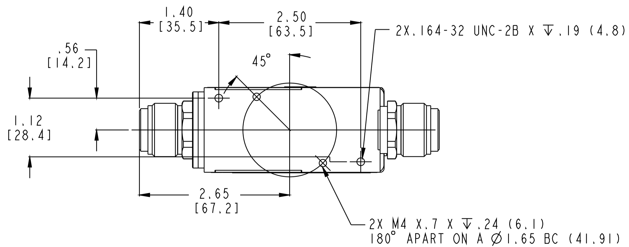
4VCR MOUNTING DIMENSIONS
