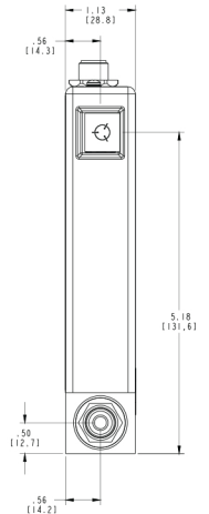
Dimensional Drawing — Normally Open (DeviceNet™ only) Unless specified, dimensions are nominal values in inches (mm referenced).
