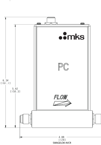
Dimensional Drawing — Normally Open (DeviceNet™ only) Unless specified, dimensions are nominal values in inches (mm referenced).
