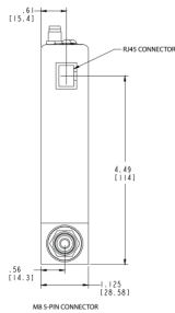
Dimensional Drawing — Normally Open (DeviceNet™ only) Unless specified, dimensions are nominal values in inches (mm referenced).
