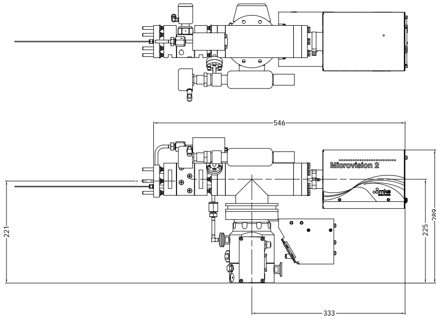
Dimensional Drawing — Unless otherwise specified, dimensions are nominal value in millimeters.
