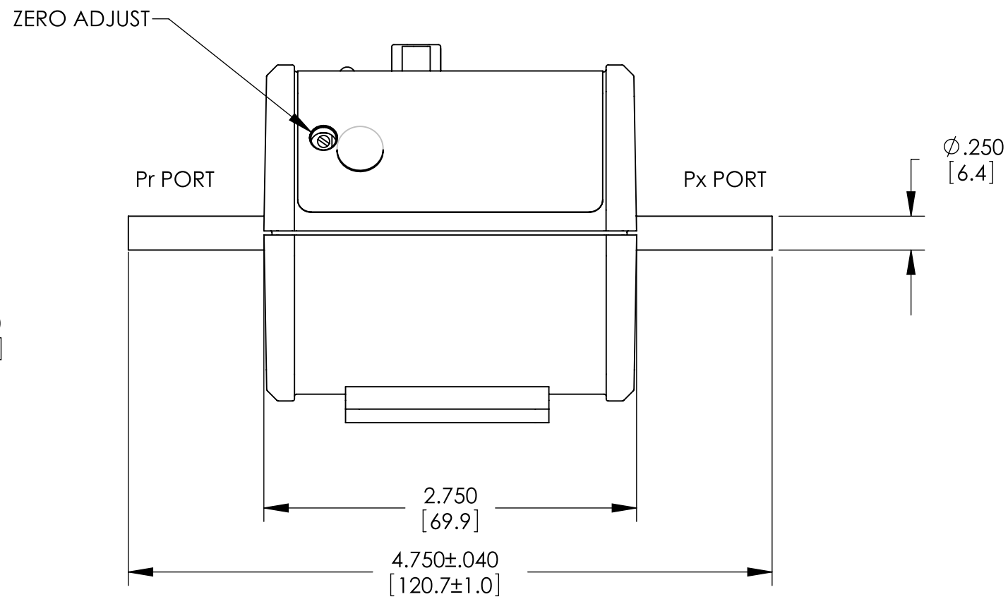
1/4" TUBE STUBS FITTING CODE BG
