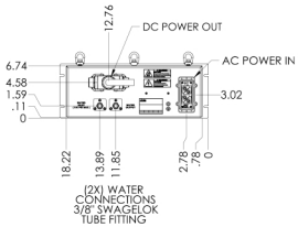
Dimensional Drawing — Unless otherwise specified, dimensions are nominal values in inches for reference only.
