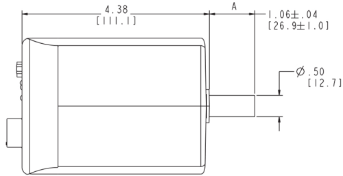
FITTING CODE -BA- Ø.50 TUBULATION
