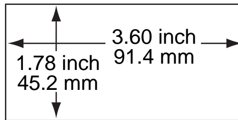
Mounting Cutout
