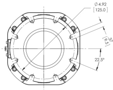
80 mm Plasma Source Dimensional Drawing. Shown with ISO80 flanges. Note: Unless otherwise specified, dimensions are nominal values in inches (mm referenced).
