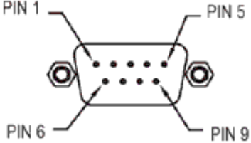
9-pin Type "D" Male Connector
