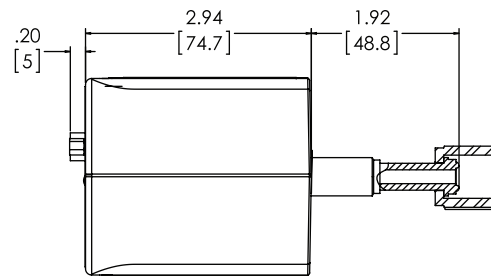
4 VCR FEMALE
