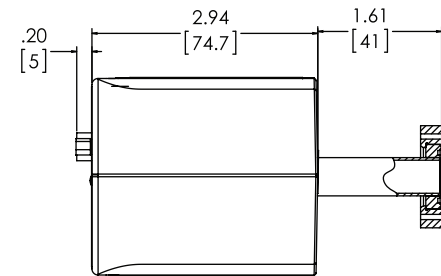
MINI-CONFLAT, ROTATABLE
