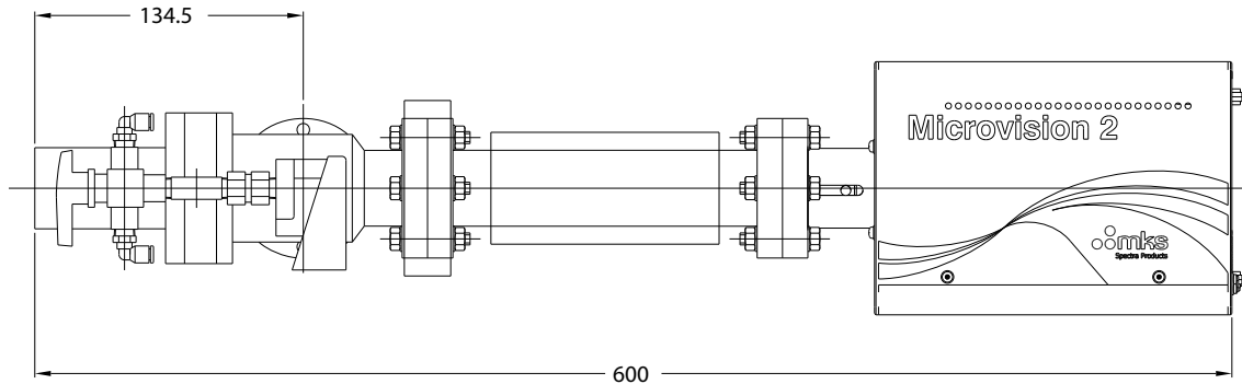
Dimensional Drawing — Note: Unless otherwise specified, dimensions are nominal values in millimeters.
