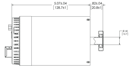
FITTING CODE -HA- 1.33 INCH CONFLAT, ROTATABLE
