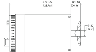
FITTING CODE -KB- 2.00 TRI-CLOVER FLANGE
