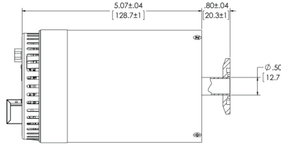
FITTING CODE -GC- NW-25-KF FACE WELD
